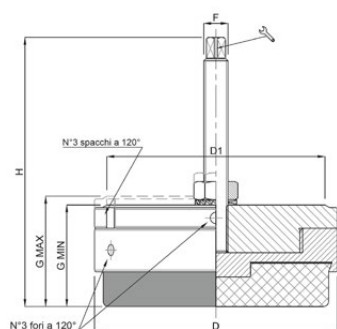
Anti moving levelling foot with fine adjustment for precise levelling
