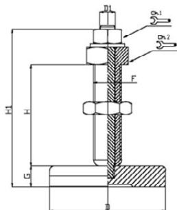
TEKNOFIX CNC Tank foot with various adjustment options
