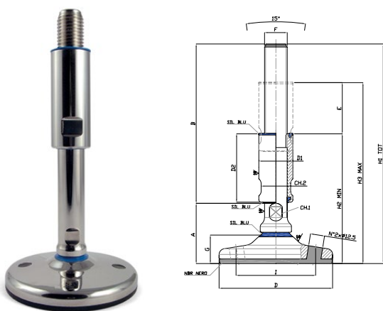
TEKNOHYGIENIC Hygienic foot with mounting holes and anti-slip in NBR black or EPDM blue
