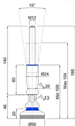
TEKNOHYGIENIC Hygienic foot with anti-slip in NBR black or EPDM blue
