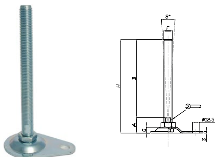
Teardrop shaped stamped levelling foot in galvanised steel with mounting holes
