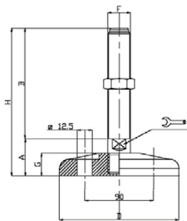
Solid stainless steel heavy duty foot with mounting holes
