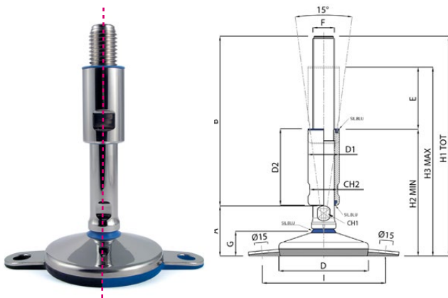
TEKNOHYGIENIC Hygienic foot with two mounting lugs and anti-slip in NBR black or EPDM blue
