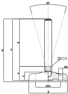
ECO Plastic foot, VA spindle - extra flat base plate with 30° levelling angle
