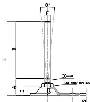
Stamped levelling foot with rectangular base and two mounting holes
