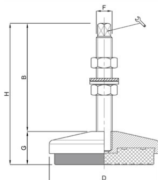
ANTIVIBRATION Heavy-duty levelling foot with vibration damping, powder-coated yellow
