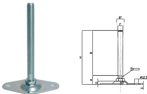
Double-drop shaped stamped levelling foot in galvanised steel with mounting holes
