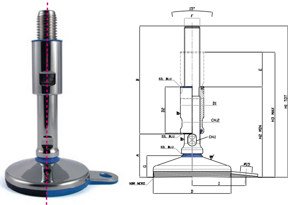
TEKNOHYGIENIC Hygienic foot with one mounting lug and anti-slip in NBR black or EPDM blue
