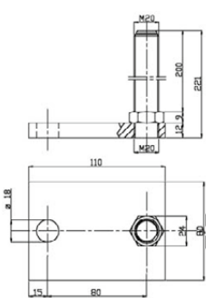
Galvanised steel foot with rectangular foot plate and fixing hole
