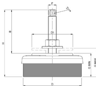
ANTIVIBRATION Heavy-duty levelling foot with vibration damping
