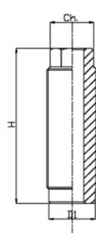
Galvanised levelling screw, with adjustment option for secure floor anchoring
