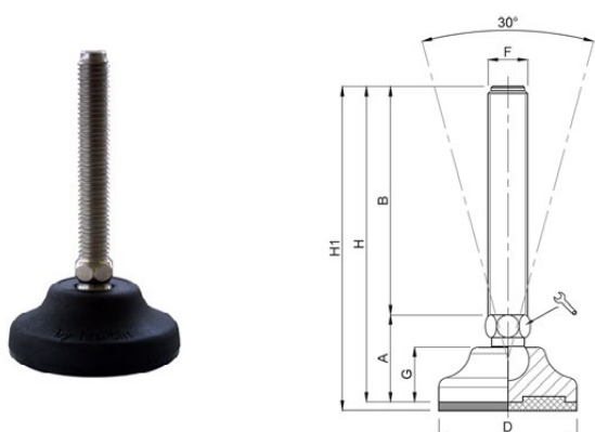
Plastic foot, VA spindle with 30° levelling angle
