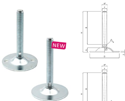
Stamped feet with or without two mounting holes
