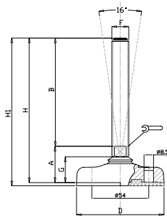
ECO Plastic foot, VA spindle - extra flat base plate with 16° spindle levelling angle
