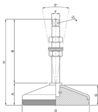
Anti vibration levelling foot with vulcanized rubber (NBR 80 shore)
