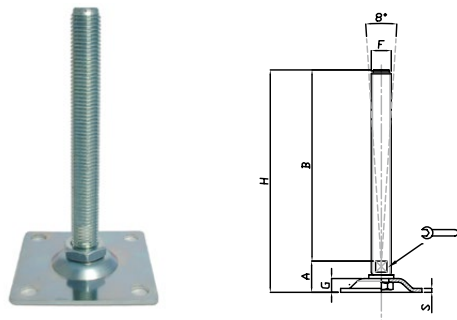
Square shaped stamped levelling foot in galvanised steel with fixing holes
