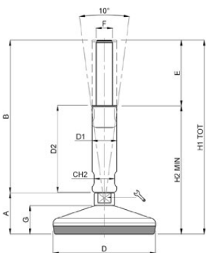
TEKNOCLEAN hygiene foot with vulcanised anti-slip plate
