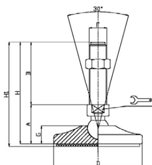
MASSIVE Steel foot, powder-coated yellow with anti-slip coating
